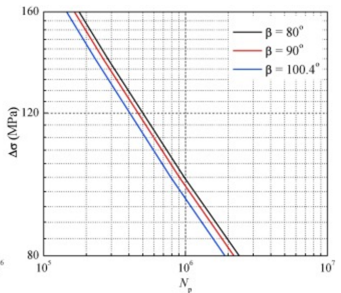
(b) D_1/t = 15 , L/t = 1.36 , a/c = 0.25 , e/t = 0.1
