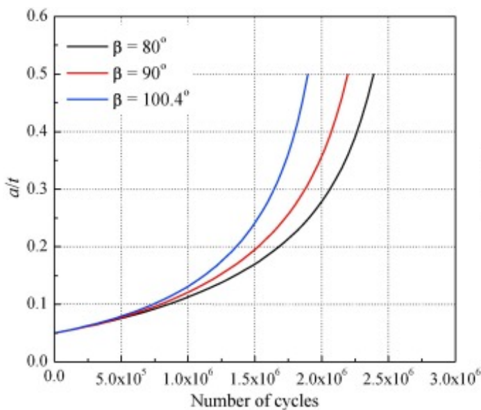
(a) D_1/t = 15 , L/t = 1.36 , a/c = 0.25 , e/t = 0.1 , \Delta\sigma = 80 MPa
